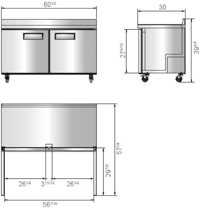
MGF8410GR
